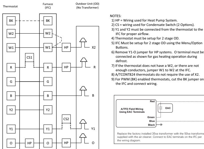
FIELD WIRING DIAGRAM FOR S9V2-VS WITH SINGLE STAGE AC OR HEAT PUMP WITH 2 STAGE AIRFLOW
