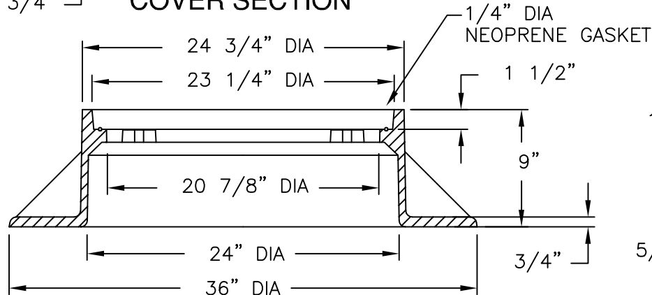
FRAME SECTION
