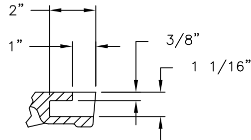
PICKHOLE DETAIL
