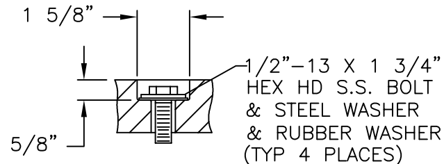
BOLT DETAIL
