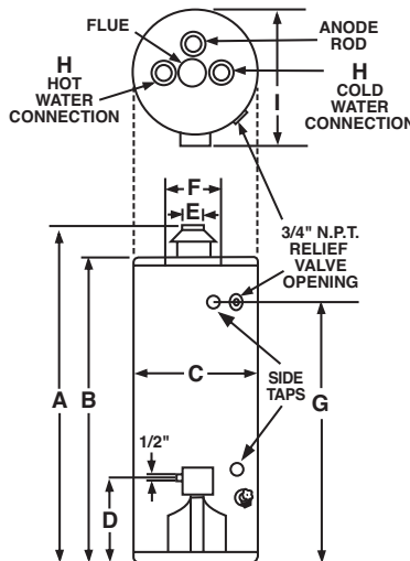
Professional Classic Heavy Duty Ultra Low NOx 75 and 98-Gallon Capacities 75,100 BTU/h Natural Gas
