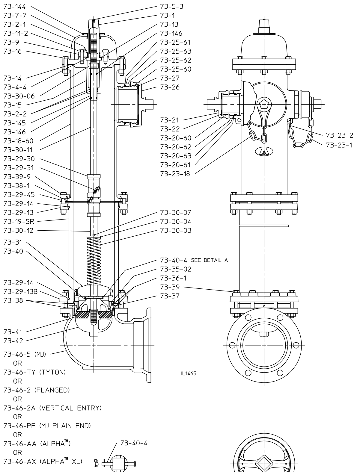
DETAIL A
