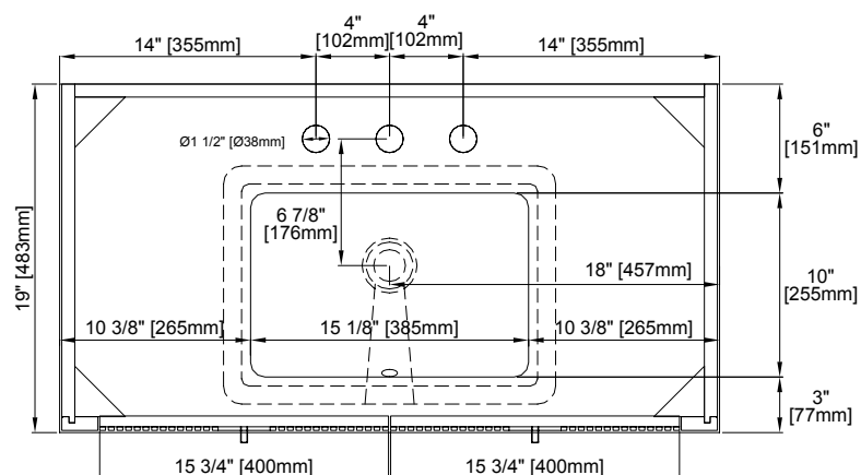
Top View
