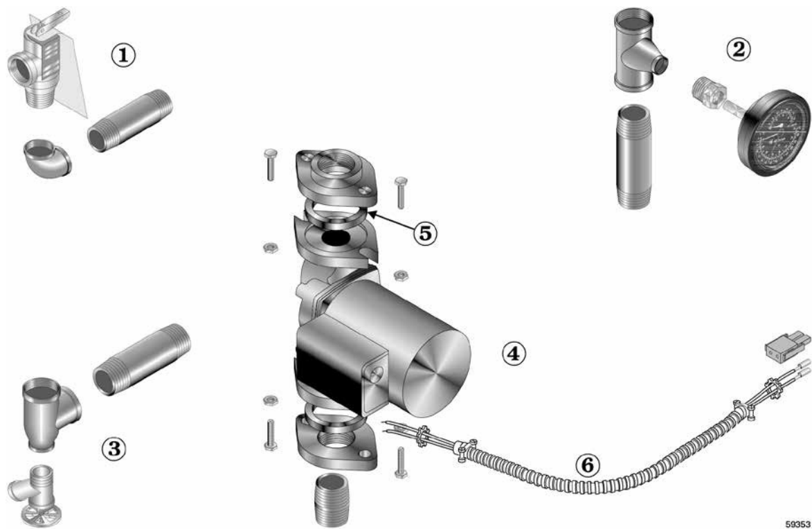
Figure 34 Trim assembly
