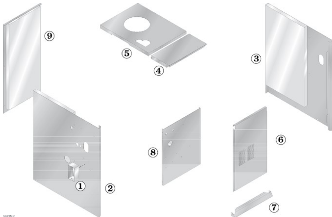
Figure 33 Jacket assembly
