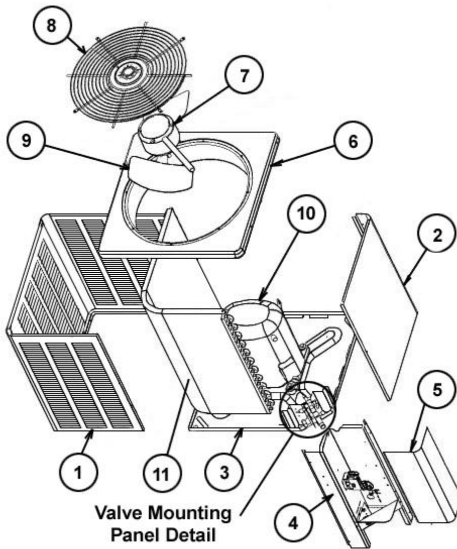
Exploded View
