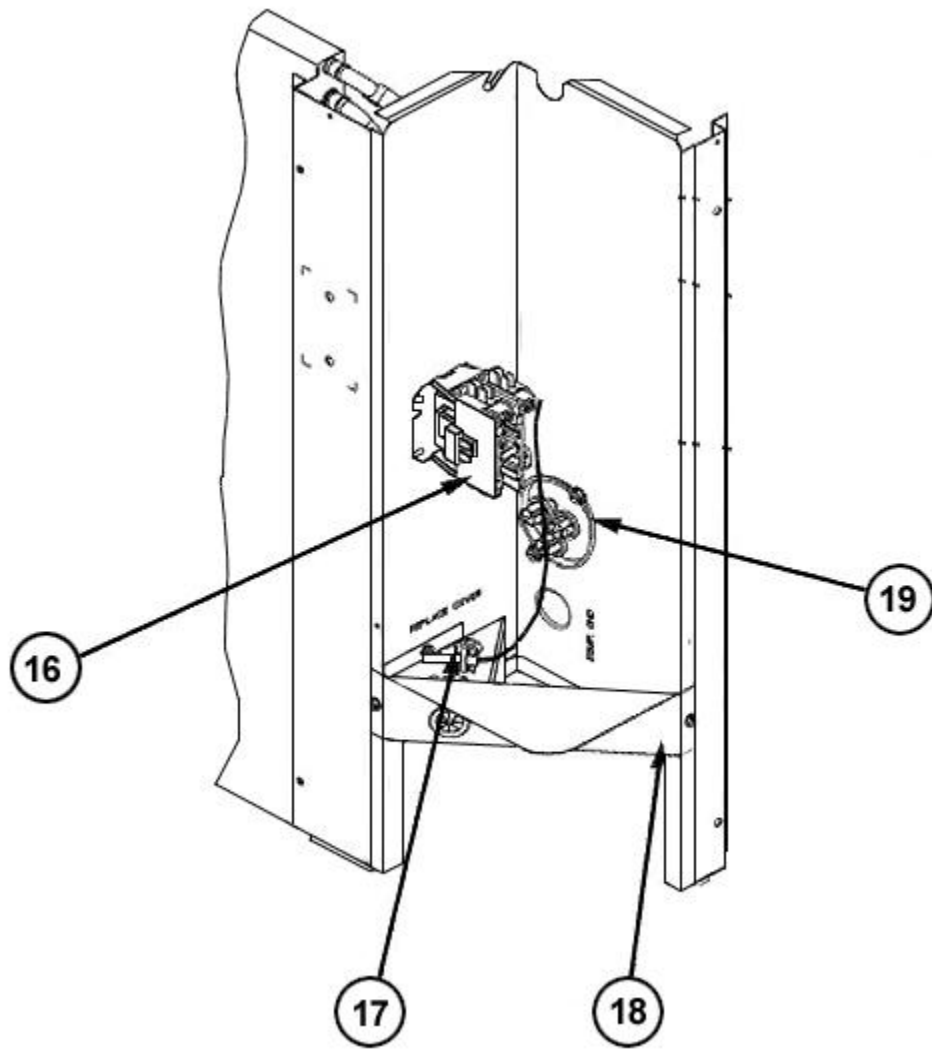
Control Box
