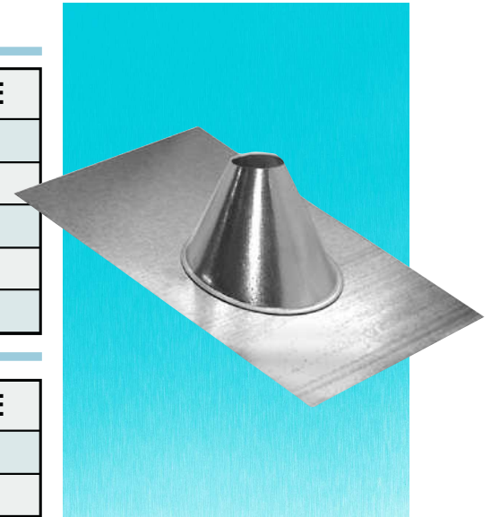
PLUMBER'S FLASHING
