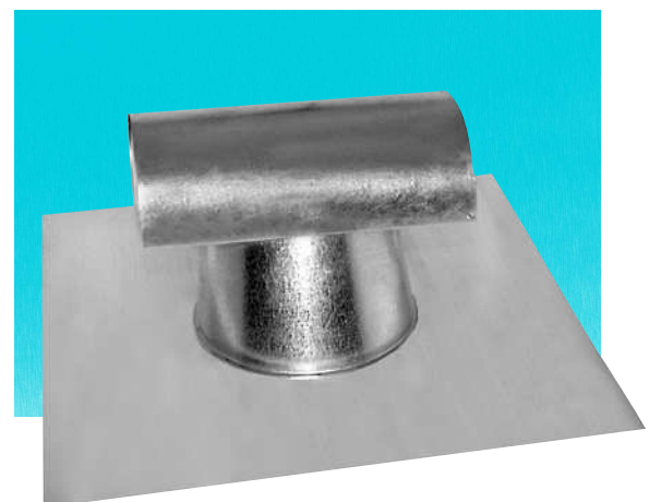
T-TOP Standard T-Tops are available on a 4/12 pitch.
