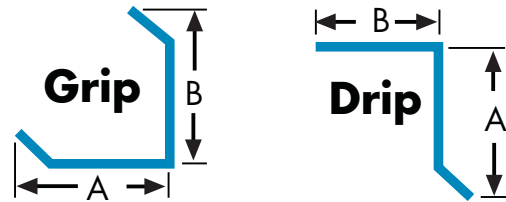
GRIP NOSING
