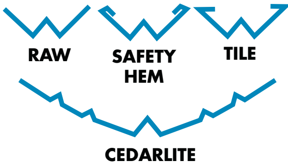
CEDARLITE VALLEY
