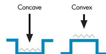
PRESSED LOUVER VENT
