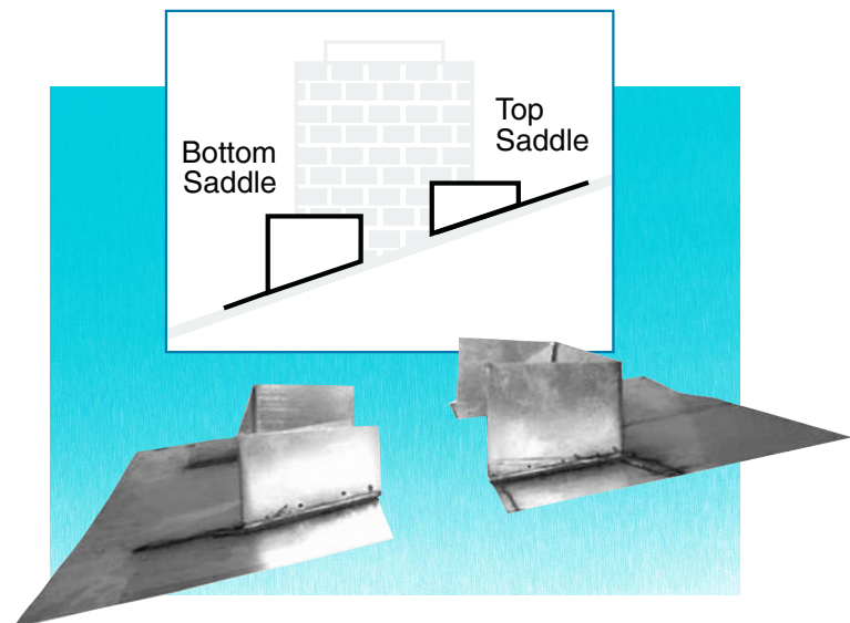
INDIVIDUAL SADDLES
