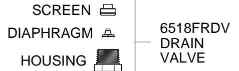
DETAIL B
