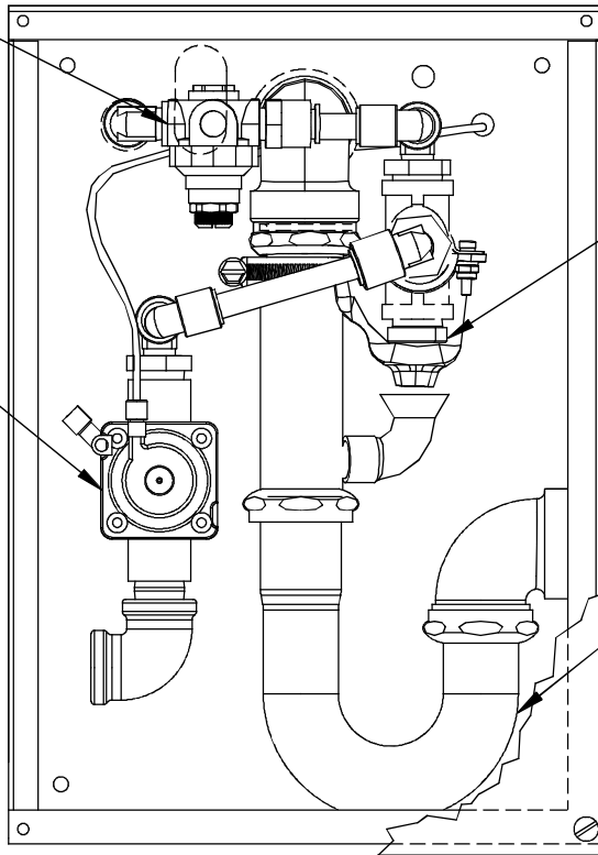
VRK3AV [1] DETAIL
