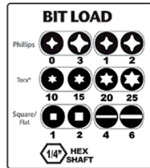
Patented Pullout Bit Cartridge
