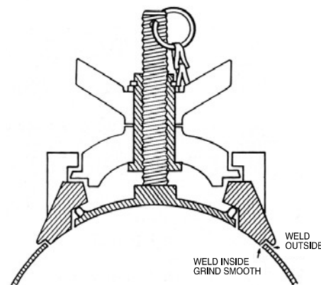
CROSS SECTION - DELUXE CLEANOUT
