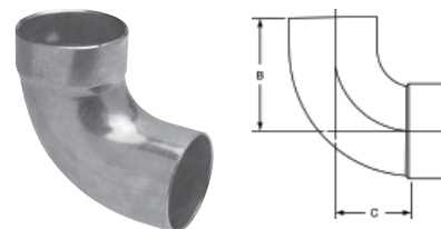
907-2 DWV 90° Fitting Elbow Ftg x C – Wrot
