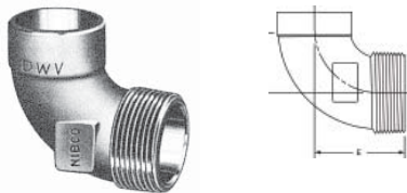
807-4 DWV 90° Elbow C x M – Cast
