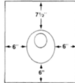
FHA Flashing
