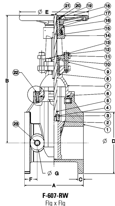
F-607-RW Flanged
