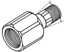
Swivel connection for misaligned pipe
