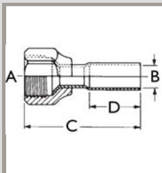
Internal FI to Extension Solder
