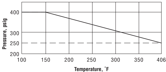
Pressure/Temperature Rating
