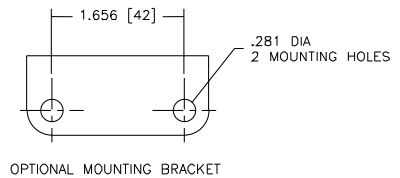
OPTIONAL MOUNTING BRACKET
