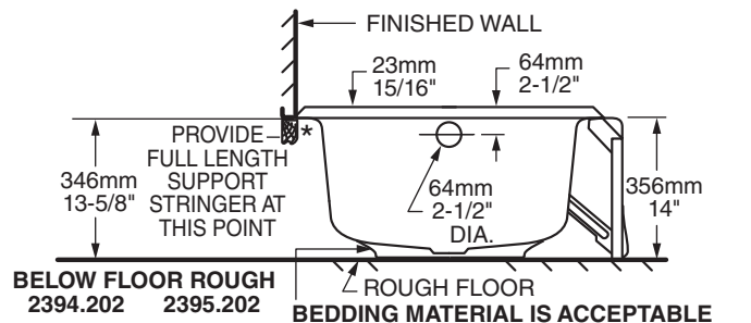
LEFT HAND TUB ILLUSTRATED RIGHT HAND TUB IS REVERSED
