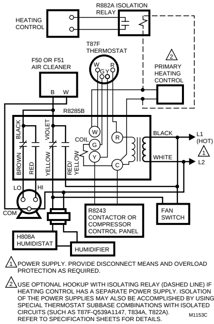
Fig. 3—R8285B typical hookup in two-speed fan motor Total Comfort application.
