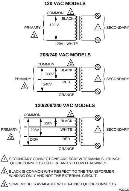
Fig. 1—Schematic for single and multitap transformers.
