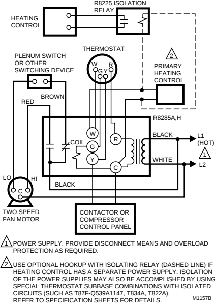
Fig. 2—R8285A typical hookup in two-speed fan motor application.
