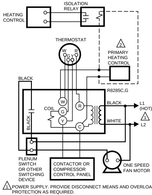
Fig. 4—R8285C,G typical hookup in one-speed fan motor application.
