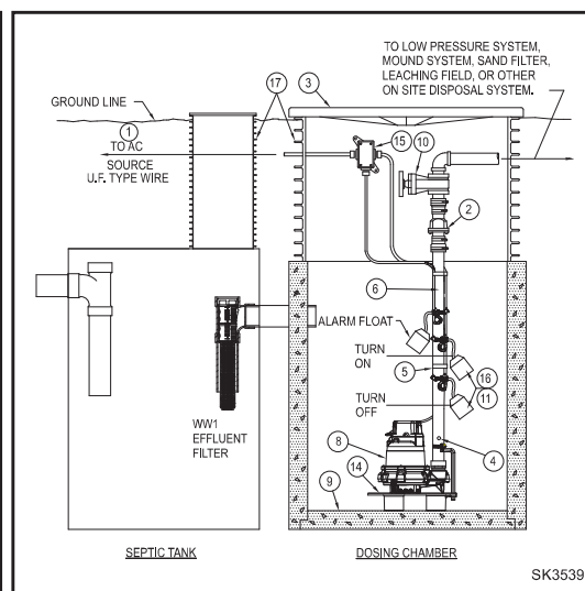
TYPICAL EFFLUENT INSTALLATION
