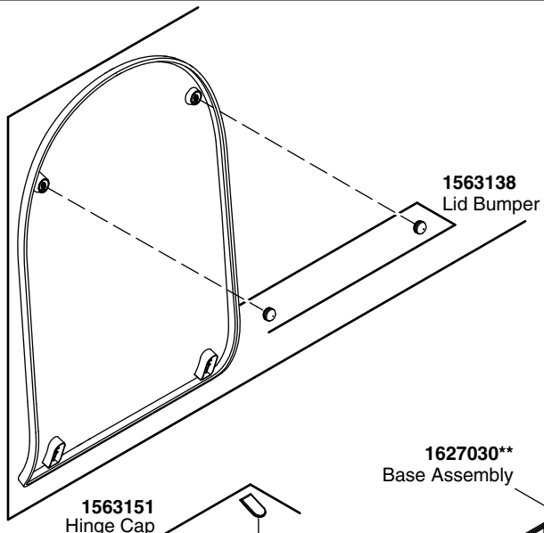
1634386** Lid Assembly
