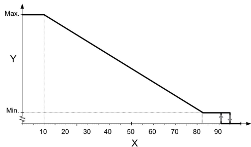
PWM input profile A (heating)
