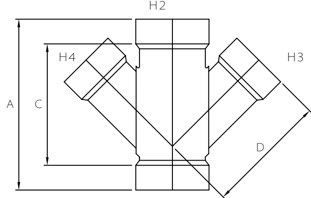
H1 FABRICATED FITTING (F)
