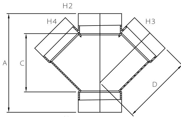
H1 INJECTION MOLDED FITTING (M)
