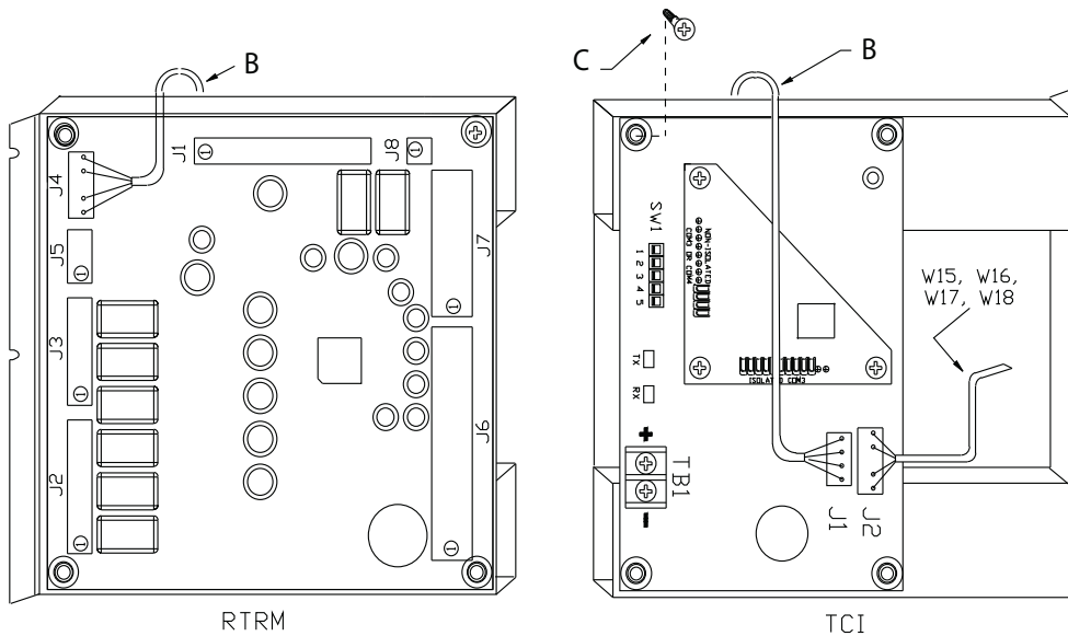
Figure 4. TCI board mounting and wiring 3 - 5 Ton packaged rooftop units (except WSC060E), 6 - 12½ ton split system units
