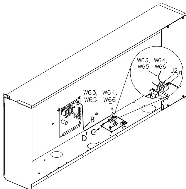
Figure 8. TCI board mounting and wiring 27 1/2 - 50 ton packaged rooftop units
