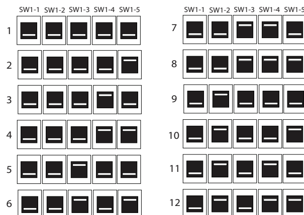
Figure 10. Comm 3/4 communications module address setting for VariTrac I comfort manager and VariTrac II central control panel — ALL address numbers and ReliaTel communications interface board DIP switch settings
