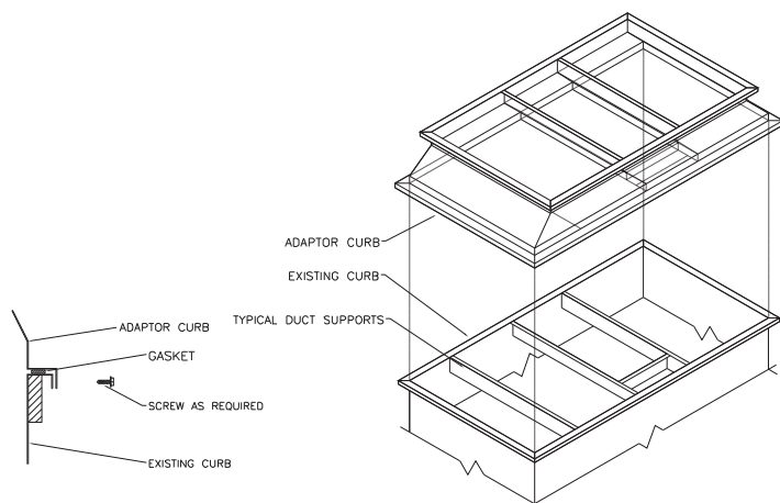
Figure 1. Curb installation
