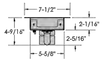
END VIEW- ALL BURNERS
