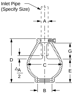
Fig. 3950T THREADED OUTLET ONLY (Specify A + B)
