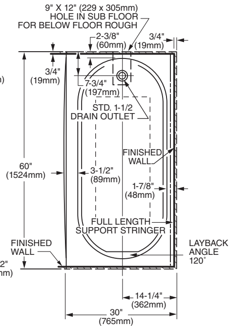
LEFT HAND TUB ILLUSTRATED RIGHT HAND TUB IS REVERSED
