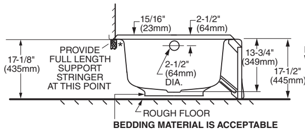
ABOVE FLOOR ROUGH 2392.202 2393.202
