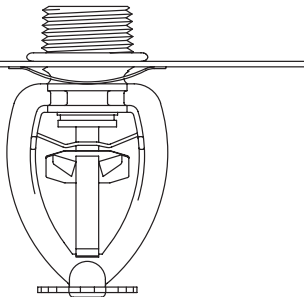
*Pendent Shown Field Assembled (Order 57-972-X-XXX Sprinkler and Shield Assembly Separately)
