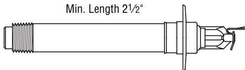
60-XXX-X-XXX Extended Coverage Sidewall w/Std. Escutcheon (1" NPT)
