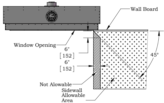
Figure 9. Combustible surrounds.
