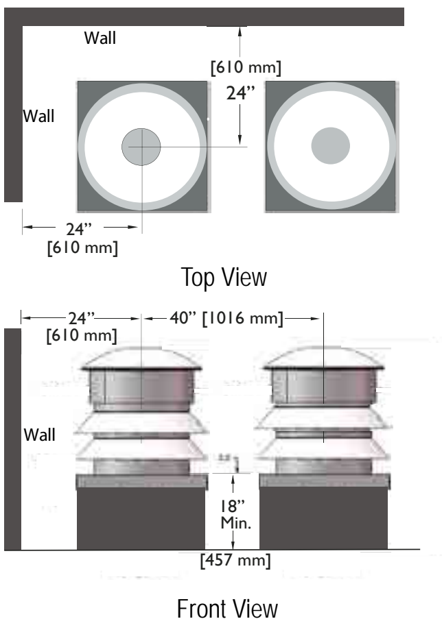
Figure 16a. PVVEX58-300 clearances
