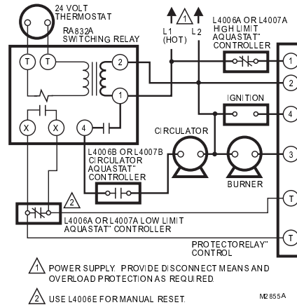
Fig. 5. Hookup for oil-fired, summer-winter, hydronic system with domestic hot water. This is typical where control for domestic hot water is added, or where each Aquastat Controller is mounted in a separate location.
