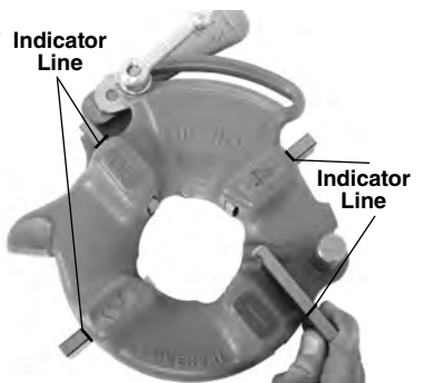
Figure 6 – Inserting Dies
