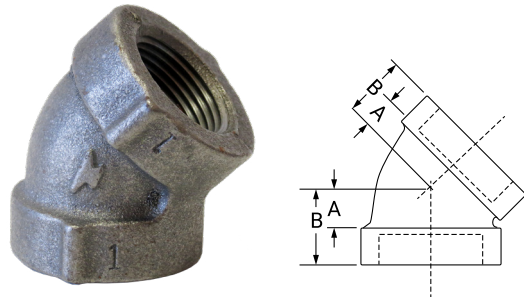
Fig. 356 45° Elbow (Straight)
