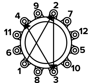
Typical Cross-Over Pattern
