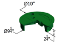
0910 T COVER HDPE
