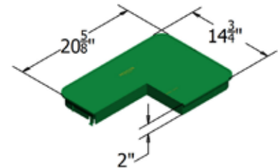
0012 T COVER HDPE
