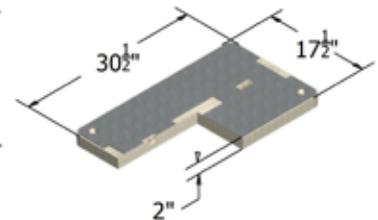
1730 FLUSH COVER POLYMER CONCRETE
