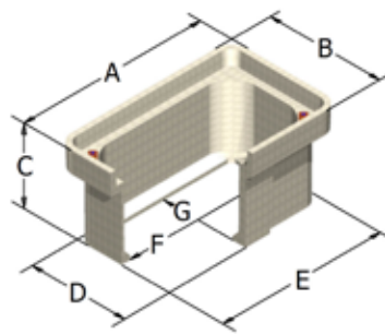
1324-12 POLYMER CONCRETE
