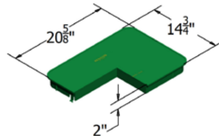
0012 T COVER HDPE
