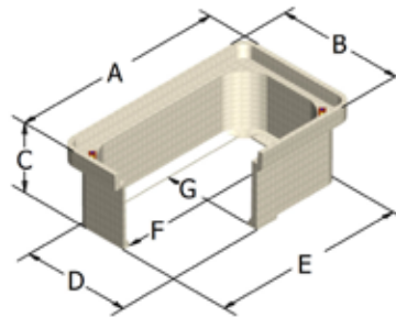
1730-12 POLYMER CONCRETE
