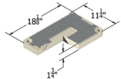
1118 COVER POLYMER CONCRETE
