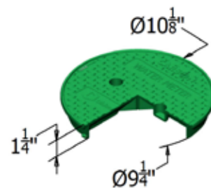
0011 T COVER HDPE
