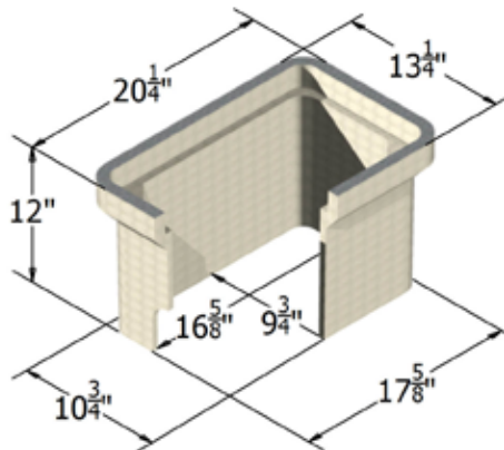
1118-12 BODY POLYMER CONCRETE
