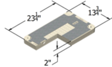
1324 FLUSH COVER POLYMER CONCRETE
