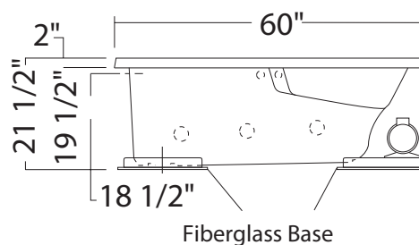
10-jet Bodywrap System SB-3260 BWS (illustrated)
