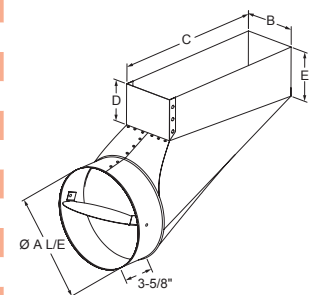
End Boot with Damper
