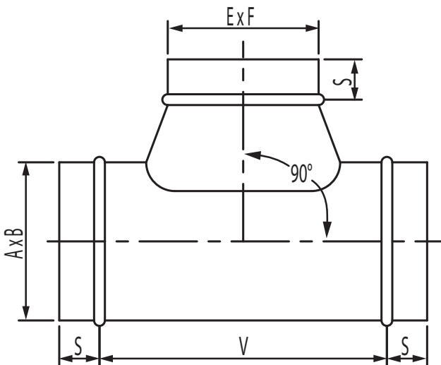
TYPE: FOCON-T-1 Conical Tee
