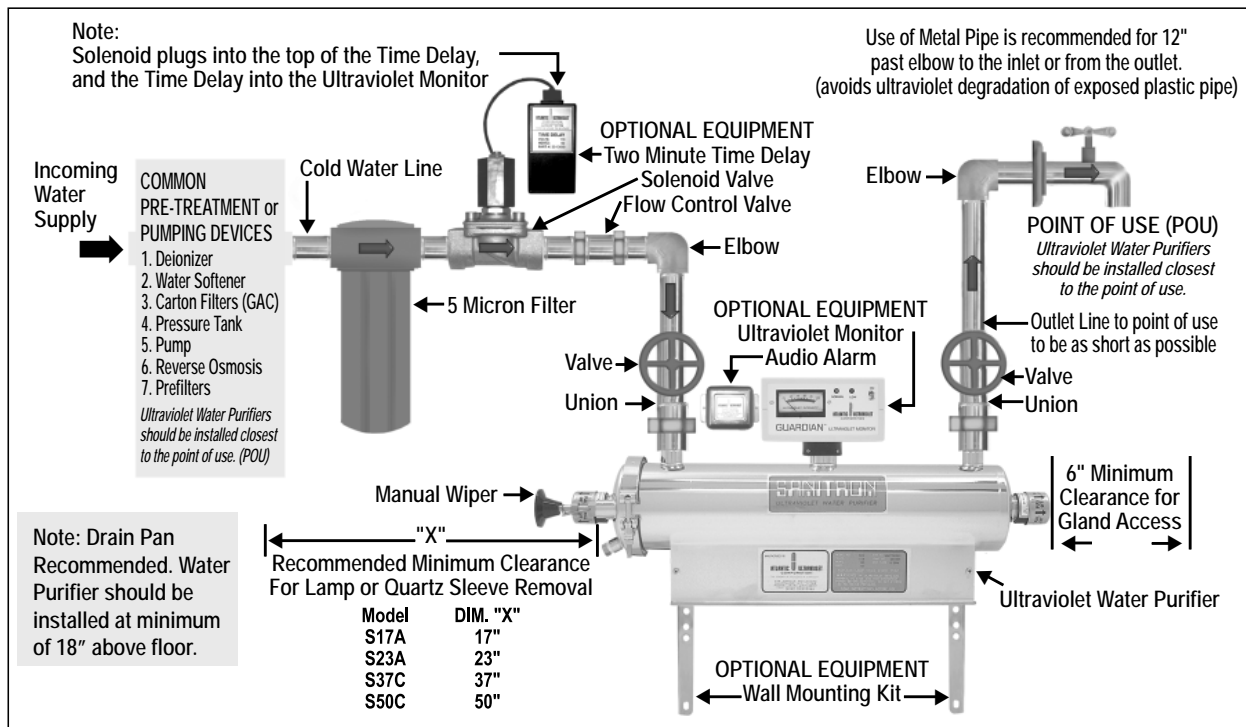
Figure 2 - Recommended Installation
