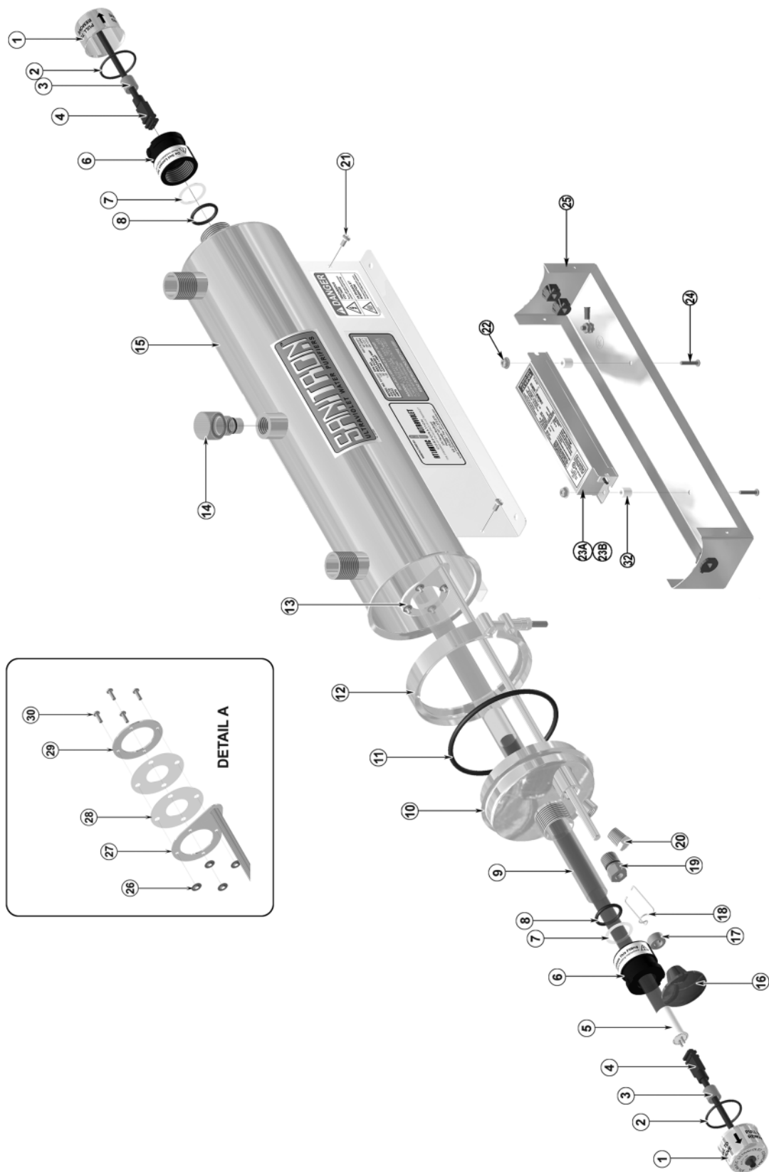
Figure 9 - Exploded View S17A & S23A
