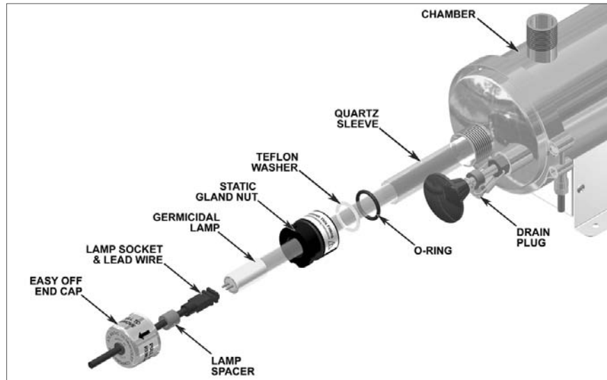
Figure 5 - Quartz Sleeve Cleaning or Replacement
