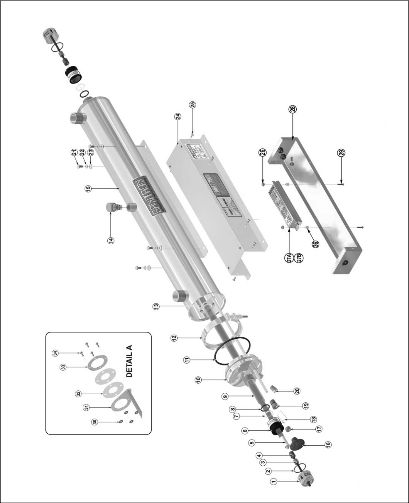
Figure 10 - Exploded View S37C & S50C
