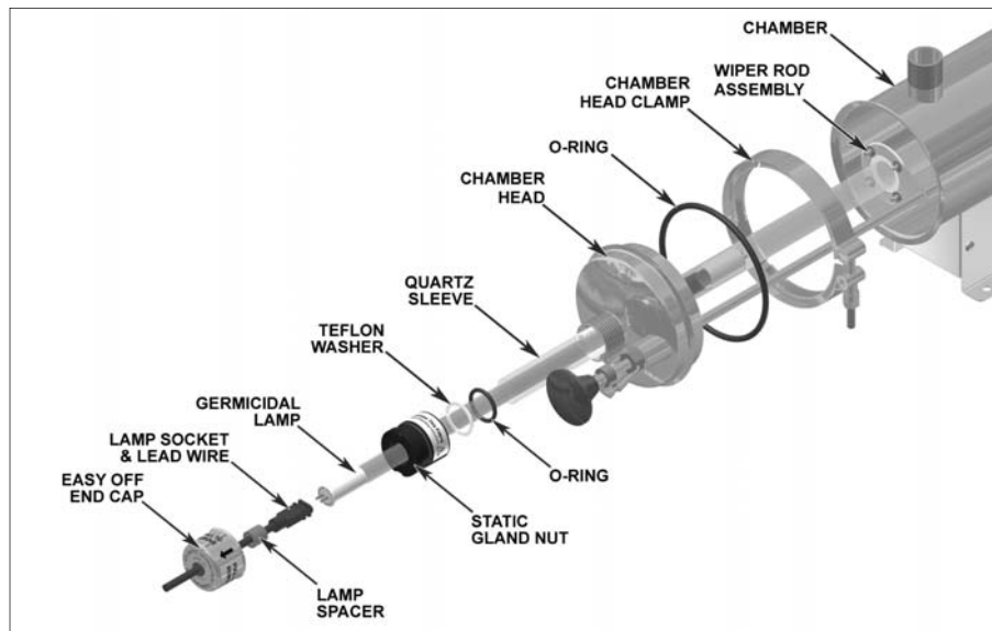
Figure 6 - Quartz Sleeve Cleaning
