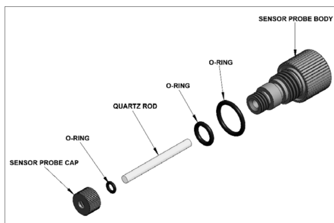
Figure 8 - Sensor Probe
