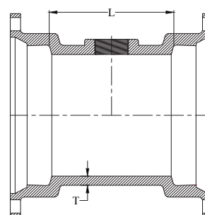
MJ TAPPED TEE (2" TAP)
