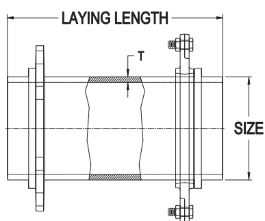
SWIVEL X SOLID ADAPTER WITH SWIVEL GLAND
