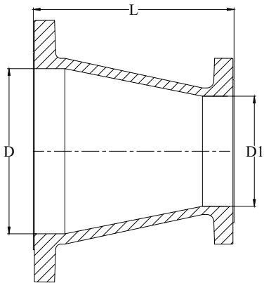
CONCENTRIC REDUCER
