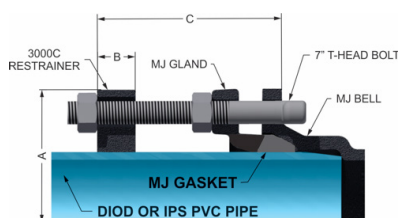
4"–12" Assembly
