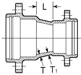
UTxUT Reducer
