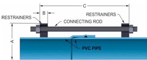
4"–12" Assembly
