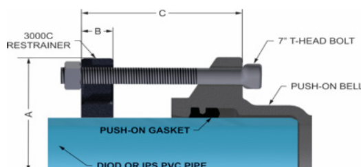
4"–12" Assembly
