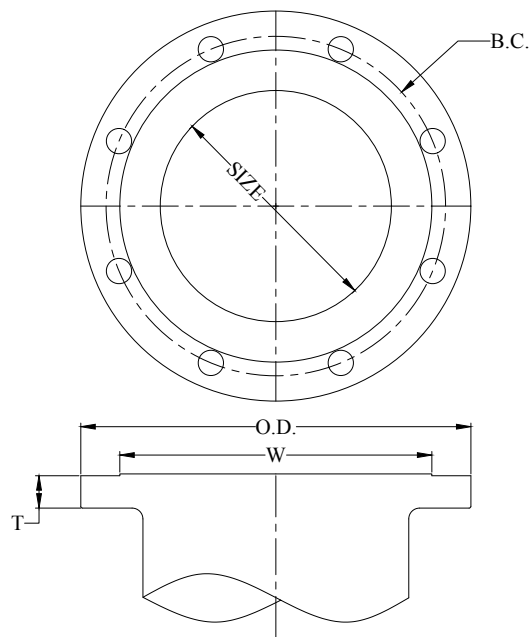
ANSI / AWWA C110 CLASS 250 FLANGE FITTINGS FLANGE DETAILS
