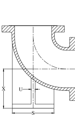
90° Base Bends
