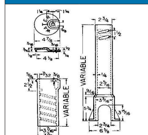
6500 SCREW TYPE CURB/SERVICE BOX
