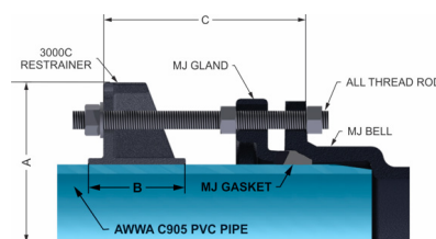
14"–36" Assembly
