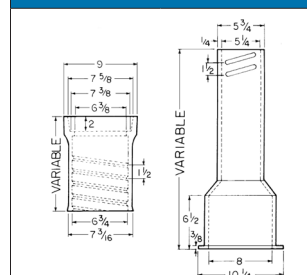
6850 SCREW TYPE VALVE BOX CAST IRON – 2 PC.
