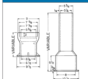
6855 SLIP TYPE VALVE BOX CAST IRON – 2 PC.
