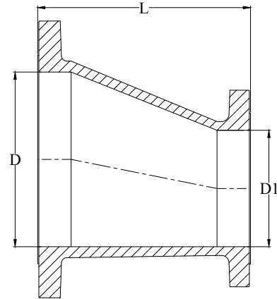
*ECCENTRIC REDUCER
