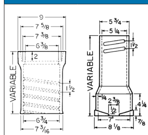
6860 SCREW TYPE VALVE BOX CAST IRON – 3 PC.
