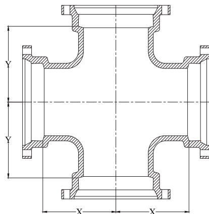
Cross
