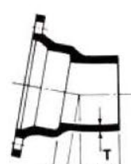
11¼° Bend
