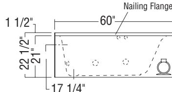
8-jet Bodywrap System OVA-4260L BWS (illustrated)
