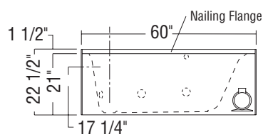
6-jet Homestead Collection OVA-4260L HMS (illustrated)
