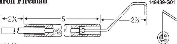
22148 LH/RH Iron Fireman 149264-G01
