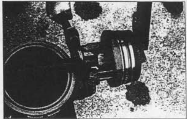
18. Hold the lower rod #32 with a pipe wrench and unscrew the valve bottom plate #45.
