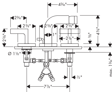
39233XX1 / 39235XX1
