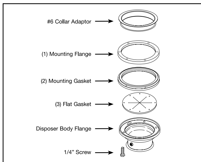
Figure 4. #6 Mounting Assembly
