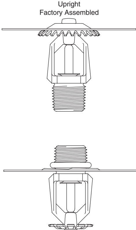
*Pendent Shown Field Assembled (Order 57-571-X-XXX Sprinkler and Shield Assembly Separately)
