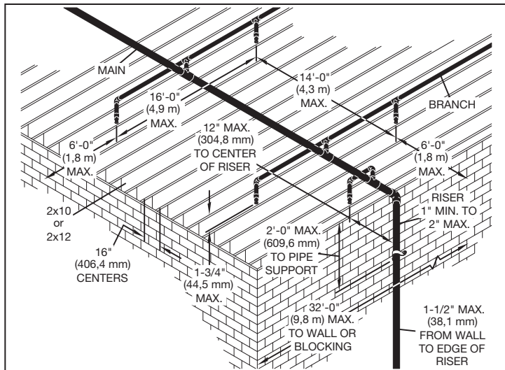
Figure 1 - Unfinished Basement, Soild Wood Joists, Center Wall Riser with Center Room Main
