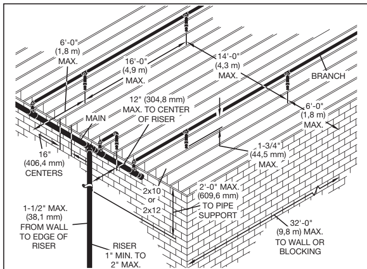
Figure 2 - Unfinished Basement, Soild Wood Joists, Center Wall Riser with Main at Wall
