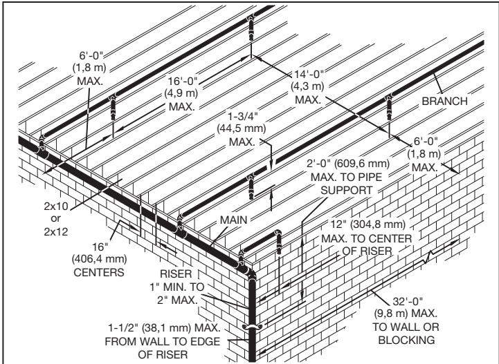
Figure 4 - Unfinished Basement, Soild Wood Joists, Blocking
