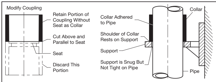
Figure 6 - Riser Collar
